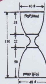
Shape & Nominal Dimensions of Combined Liquor Measures 60 ml. & 30 ml.
